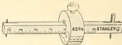
Marking Gauge.
